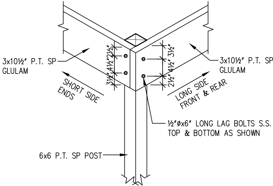
8 R10 GLULAM/END POST CONNECTION: 3/4"=1'-0"
