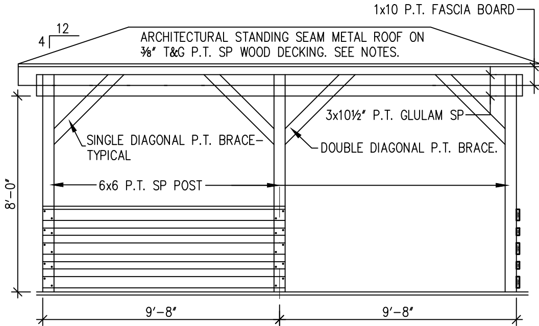
NORTH ELEVATION: 1/4"=1'-0" SOUTH (OCEAN SIDE)
