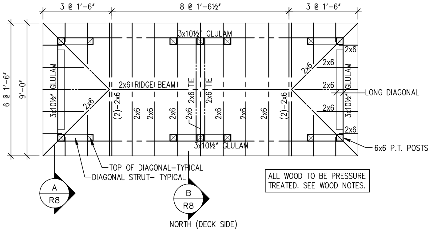
ROOF FRAMING PLAN 1/4"=1'-0"
