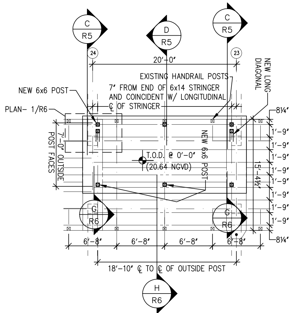
PLAN- VIEW: 1/8"=1'-0"
