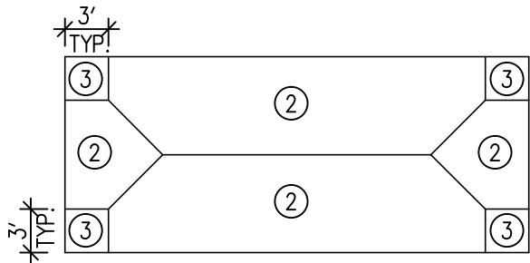
ROOF PLAN- WIND PRESSURE LOADS
