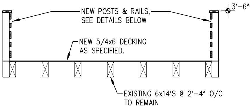
DETAIL 1 1/4"=1'-0"
