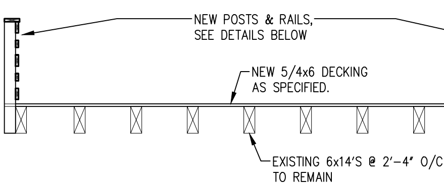
DETAIL 2 1/4"=1'-0"
