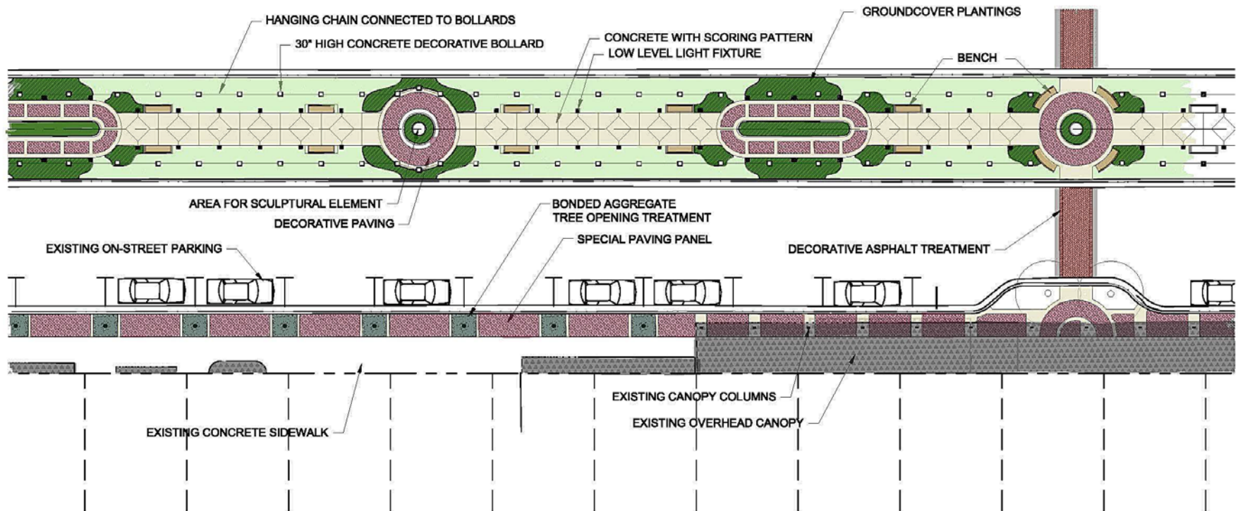
PROPOSED HARDSCAPE DEVELOPMENT WITH CONCRETE BOLLARD AND CHAIN J-WALKING DETERANTS
