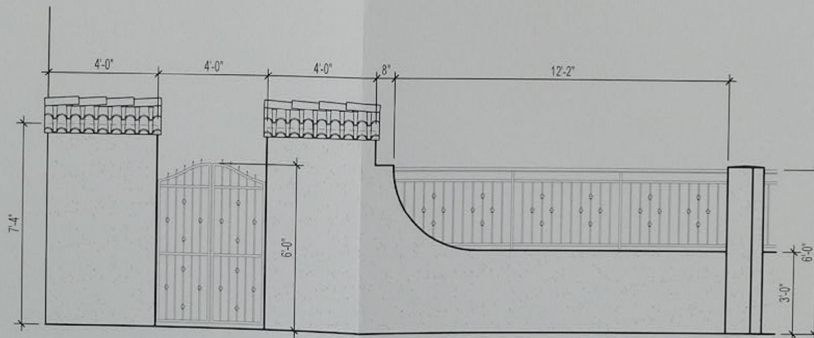
ENLARGED NORTH WALL ELEVATION
