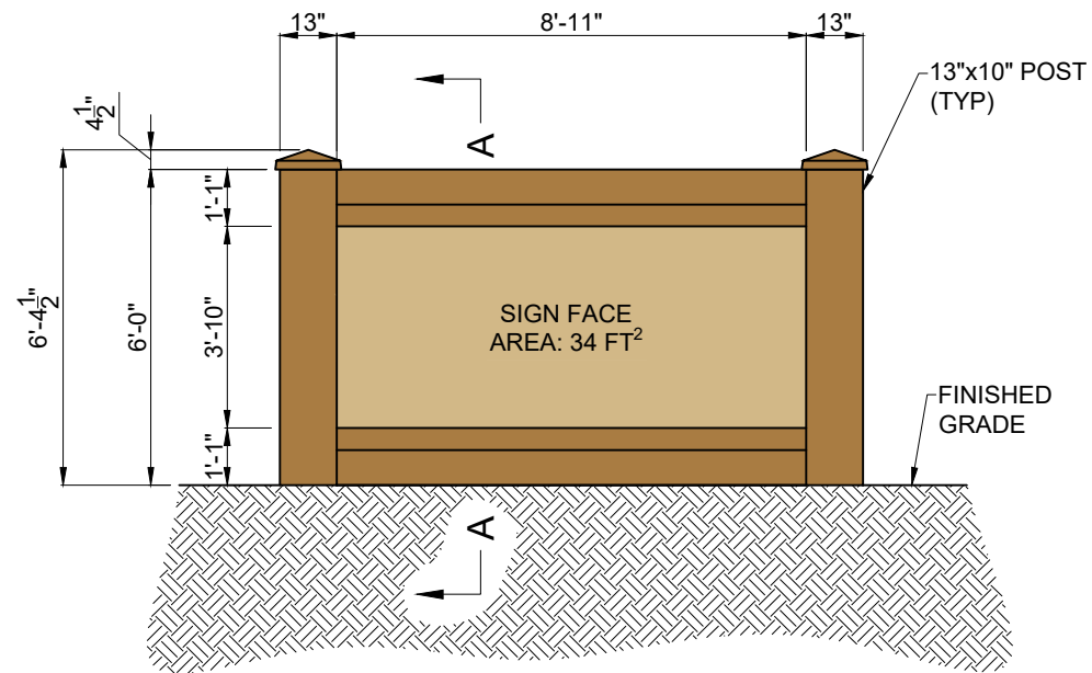
FRONT ELEVATION VIEW SCALE: \frac{3}{16}" = 1'-0"
