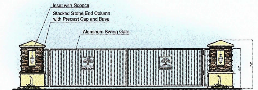
A2 ENTRY GATE CONCEPT Scale 1/4" = 1'-0"
