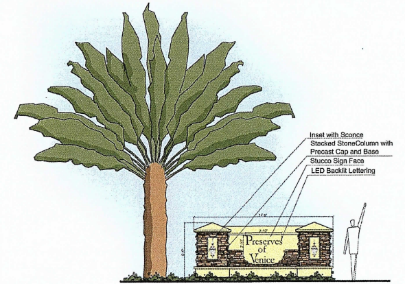
A1 ENTRY SIGN CONCEPT Scale 1/4" = 1'-0"
