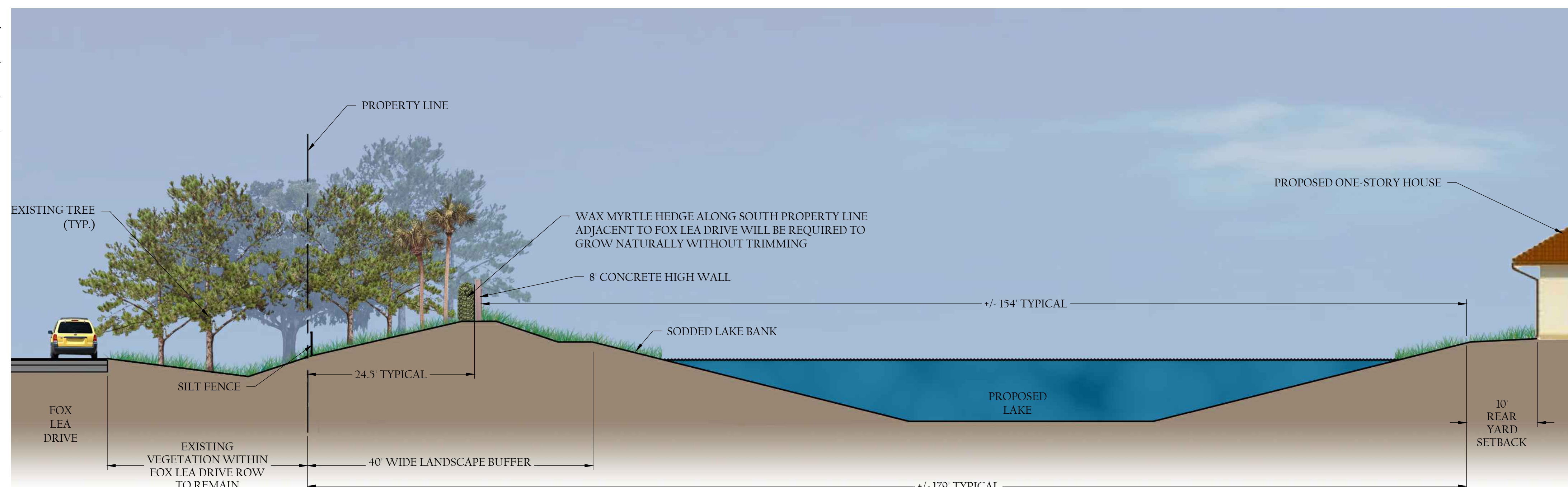
FOX LEA DRIVE TYPICAL LANDSCAPE BUFFER & SETBACKS SECTION
