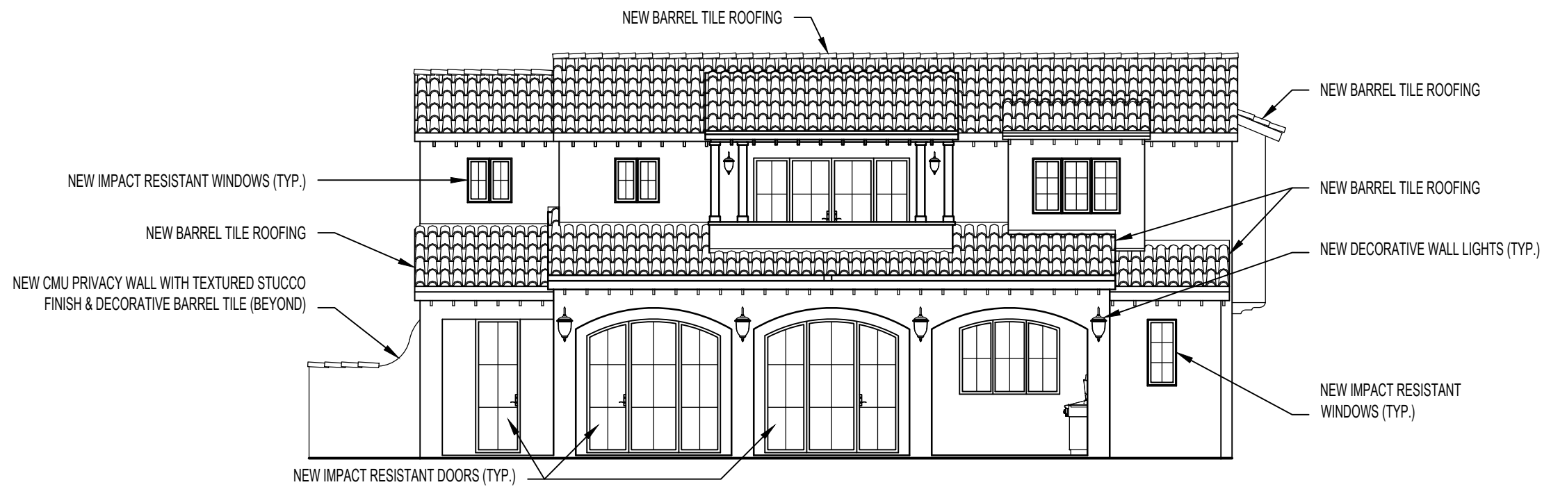
East Elevation
