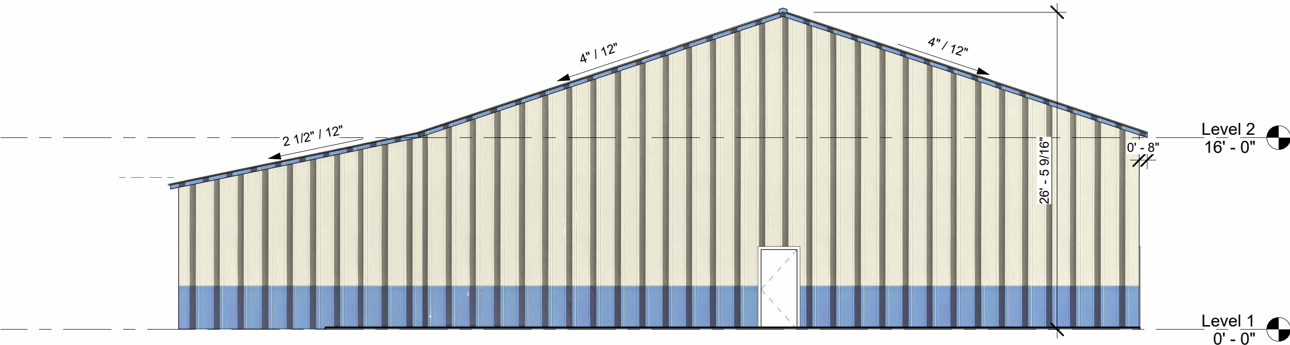
③ Left 1/8" = 1'-0"
