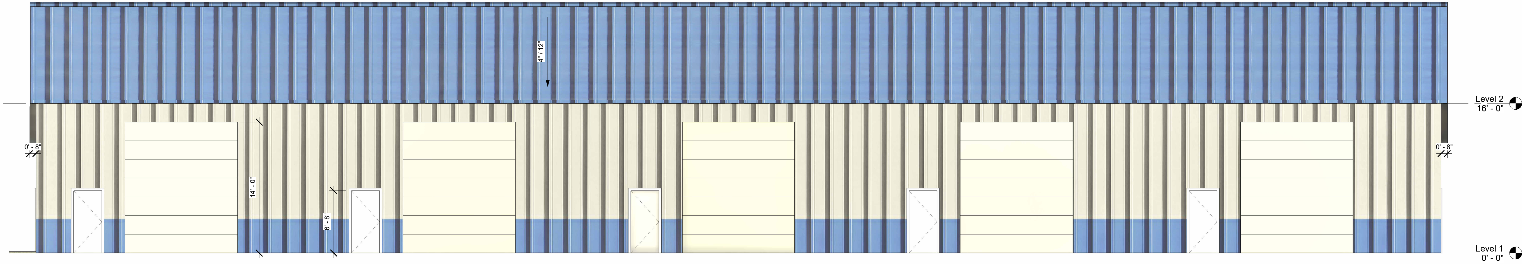
① Front 3/16" = 1'-0"
