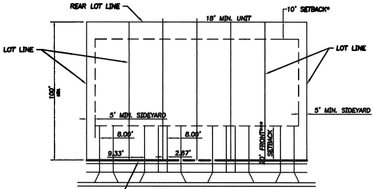
TYPICAL LOT DETAIL 4/6 UNIT TOWNHOME BUILDING
