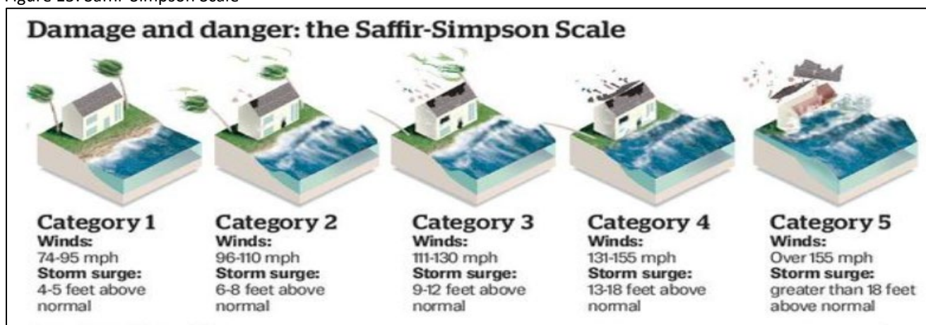
Figure 15: Saffir-Simpson Scale
