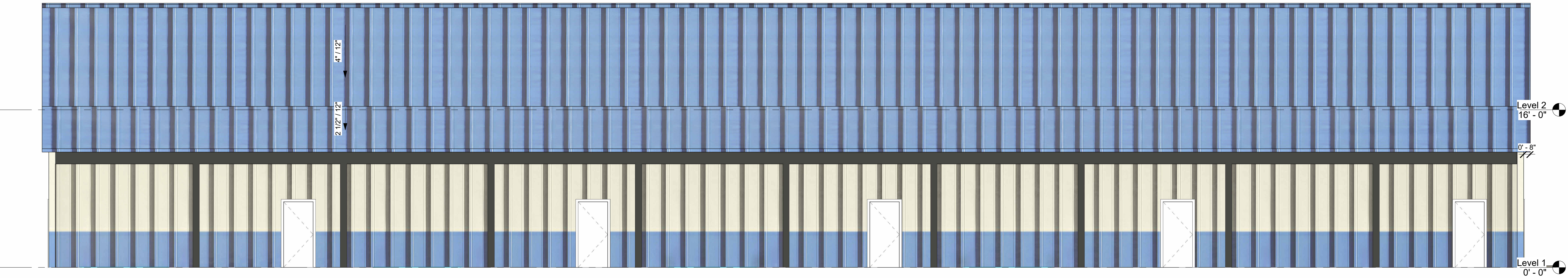
② Back 3/16" = 1'-0"
