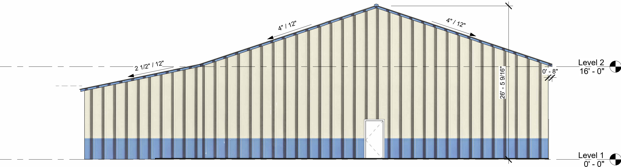
③ Left 1/8" = 1'-0"
