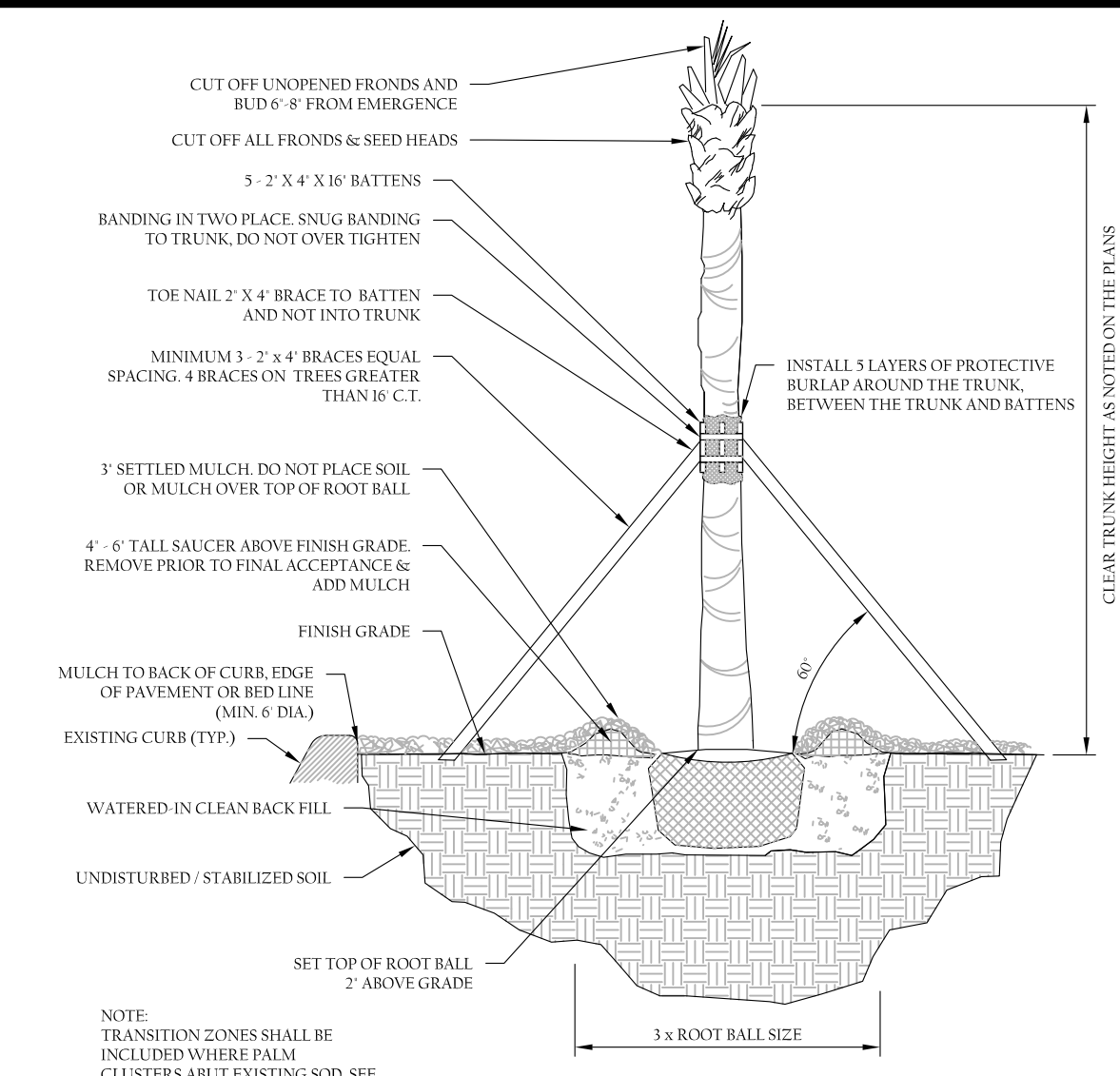
SABAL PALM PLANTING DETAIL
