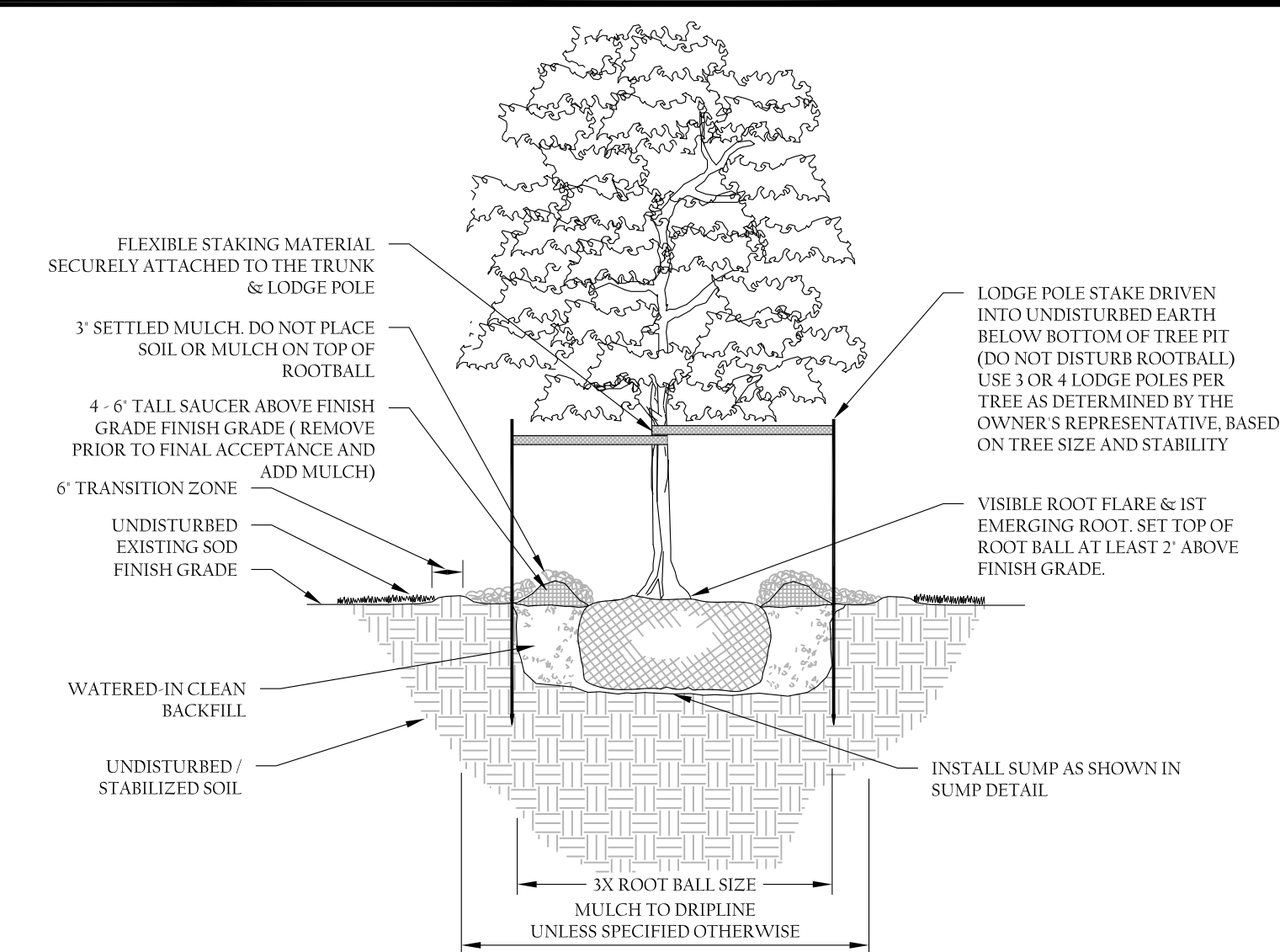
SINGLE TRUNK TREE PLANTING DETAIL
