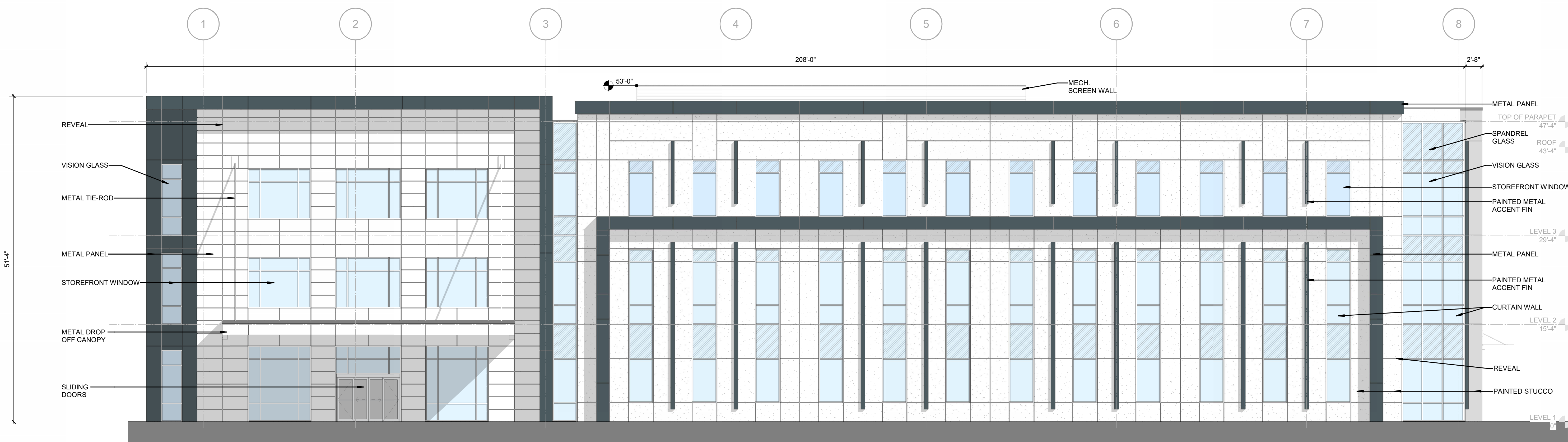
1 ELEVATION- EXTERIOR- SOUTH AP-209 1/8" = 1'-0"
