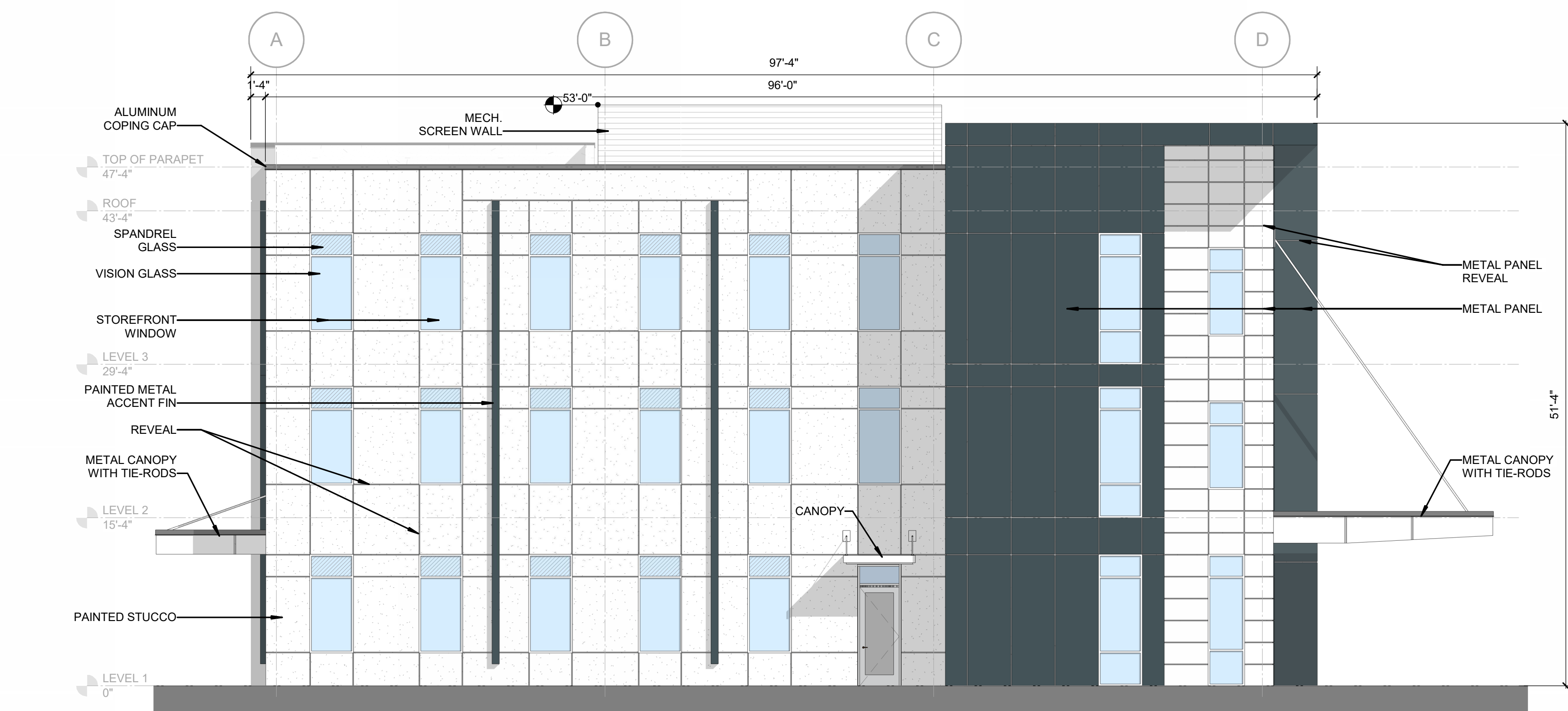
3 ELEVATION- EXTERIOR- WEST AP-209 1/8" = 1'-0"
