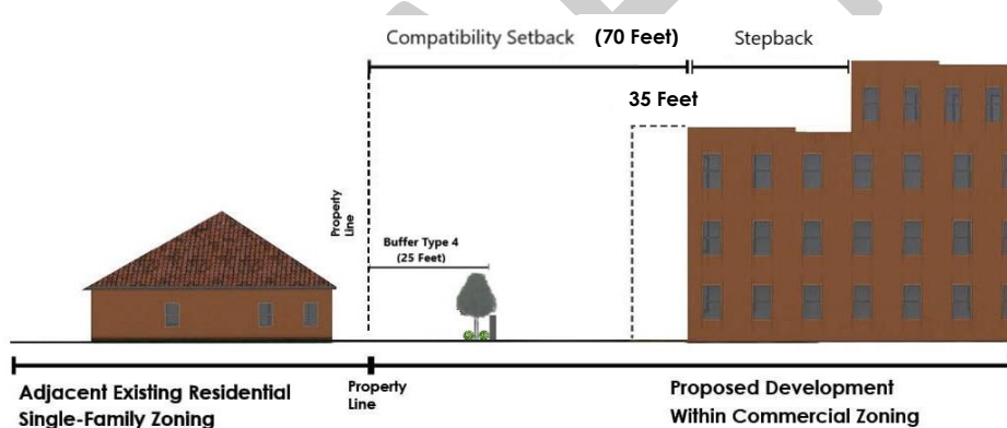
Figure 4.5.1. Step-back, Buffer, and Compatibility Setback
