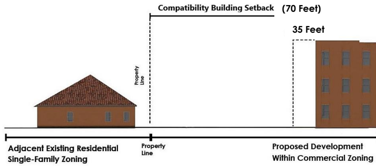
Figure 4.2. Compatibility Building Setback Example
