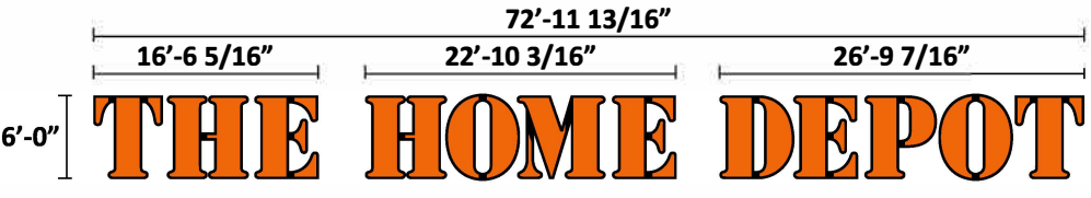
A 6'-0" CHANNEL LETTERS: 437.91 Square Feet
