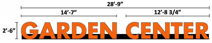
B 2'-6" CHANNEL LETTERS ON BOTTOM MOUNT RACEWAY: 71.88 Square Feet
