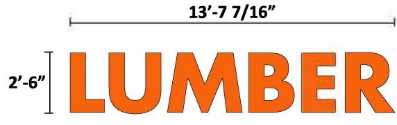
C 2'-6" CHANNEL LETTERS: 34 Square Feet
