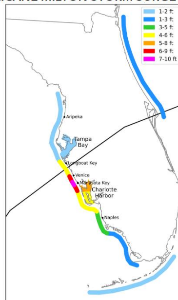
HURRICANE MILTON STORM SURGE (AGL)
